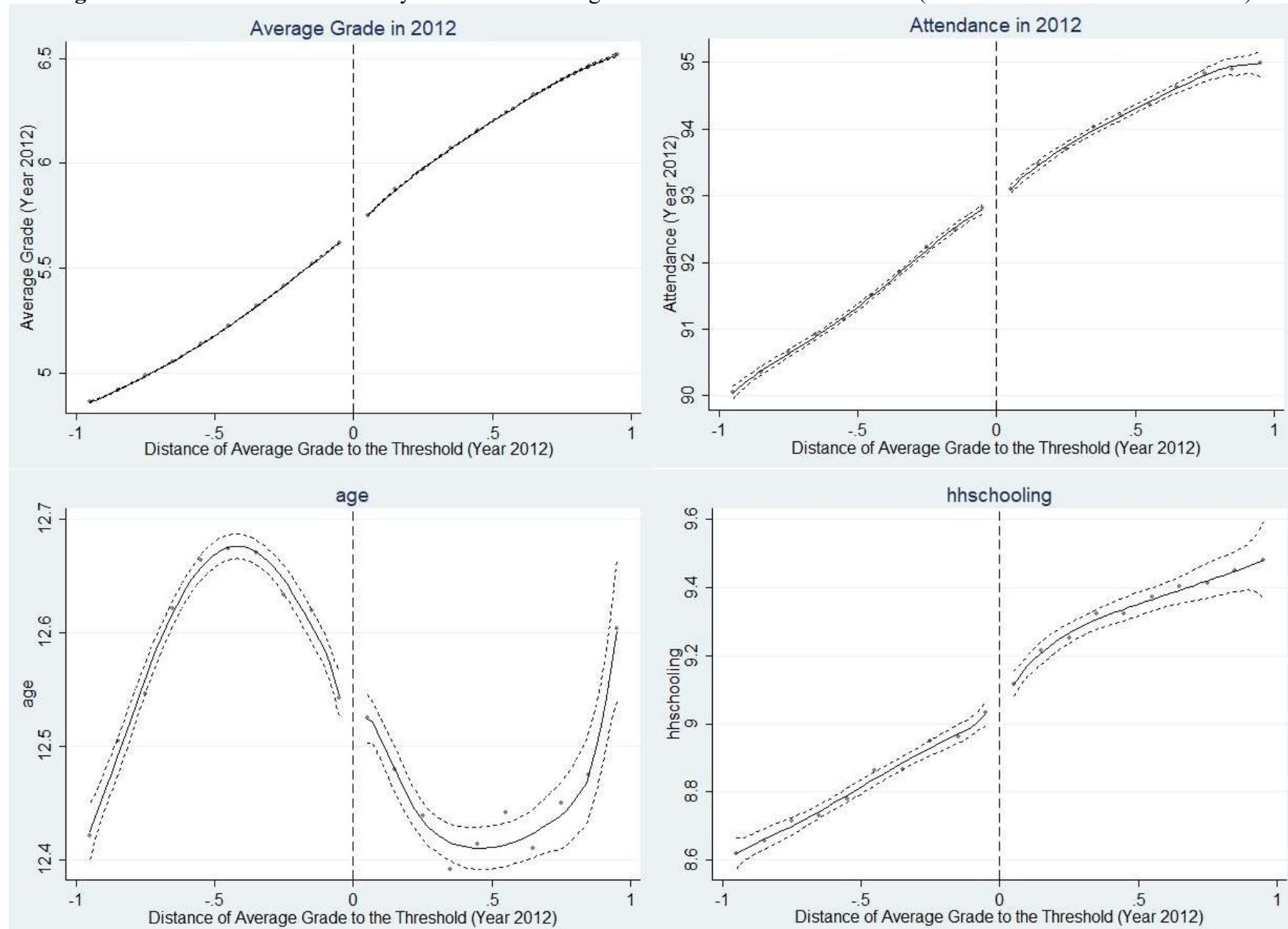
Figure 6: Pre-Treatment Variables by Distance of Average Grade to the Threshold in 2012 (Students with PFSE \leq 98 in 2012)
