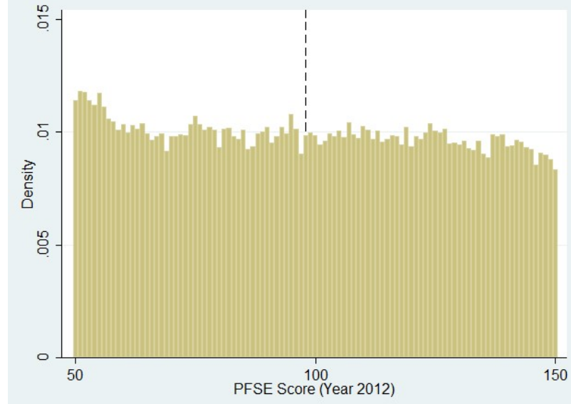
Figure 1: PFSE Score Density and Frandsen Manipulation Test (Students in the Highest 30% of Academic Performance in 2012)
