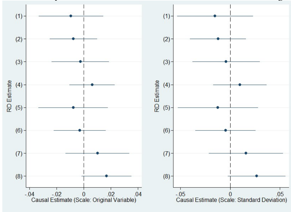
Figure 7: Summary of RD Point Estimates and Confidence Intervals for Average Grade
