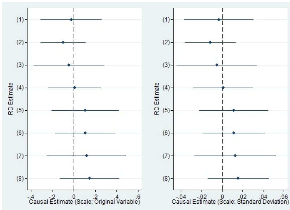
Figure 8: Summary of RD Point Estimates and Confidence Intervals for Attendance
