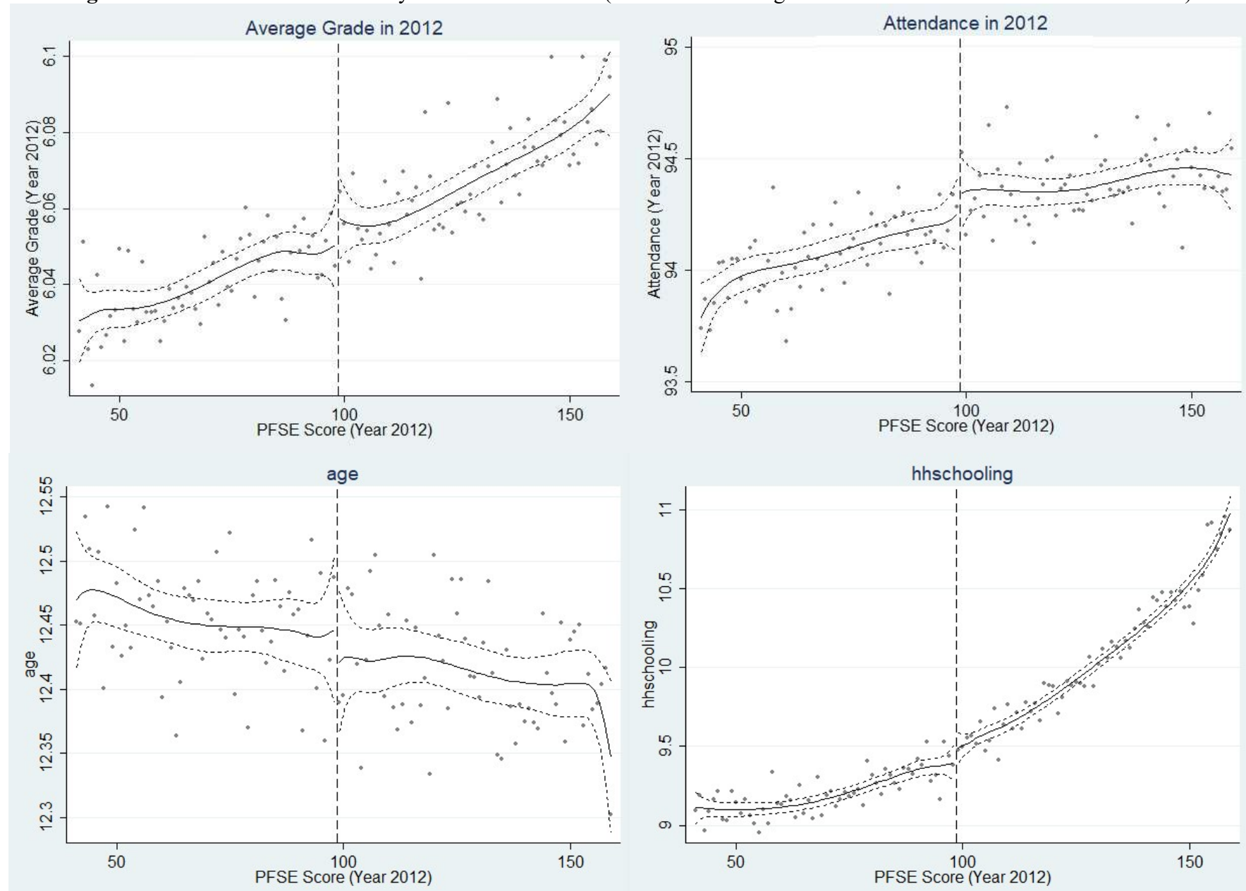
Figure 3: Pre-Treatment Variables by PFSE Score in 2012 (Students in the Highest 30% of Academic Performance in 2012)
