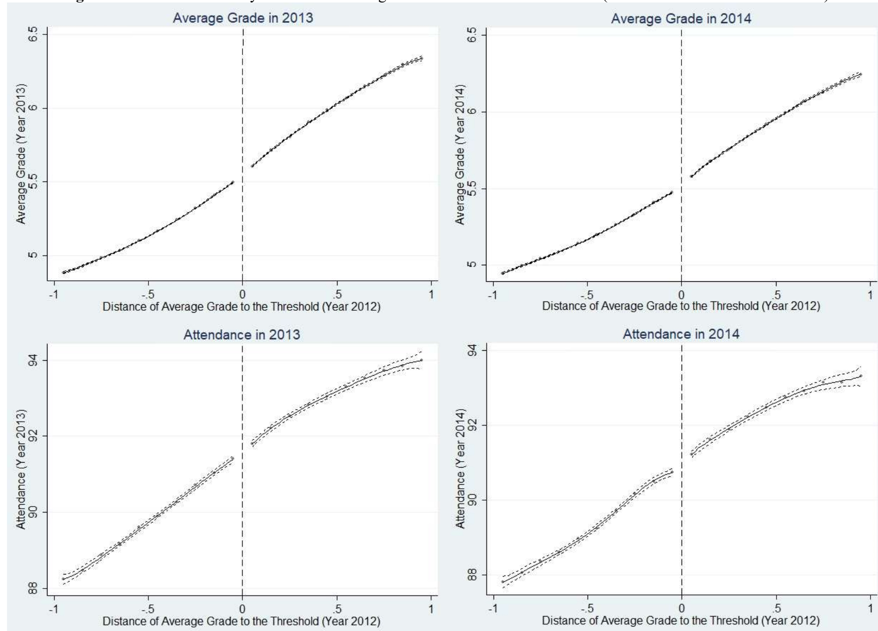
Figure 5: Future Outcomes by Distance of Average Grade to the Threshold in 2012 (Students with PFSE \leq 98 in 2012)
